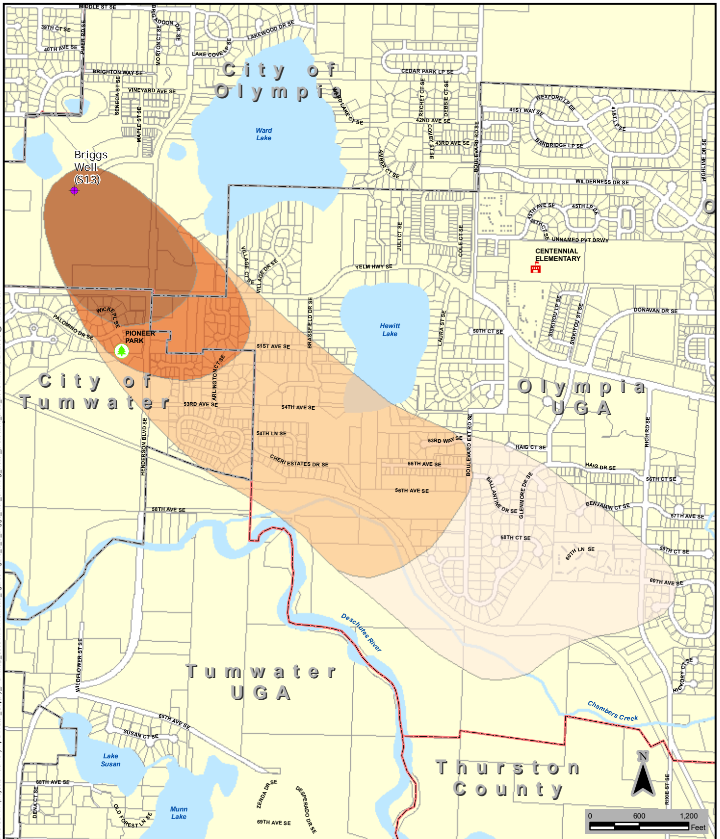
FIGURE 8.8 Briggs Well Drinking Water Protection Area, 2008 2009 Water System Plan
